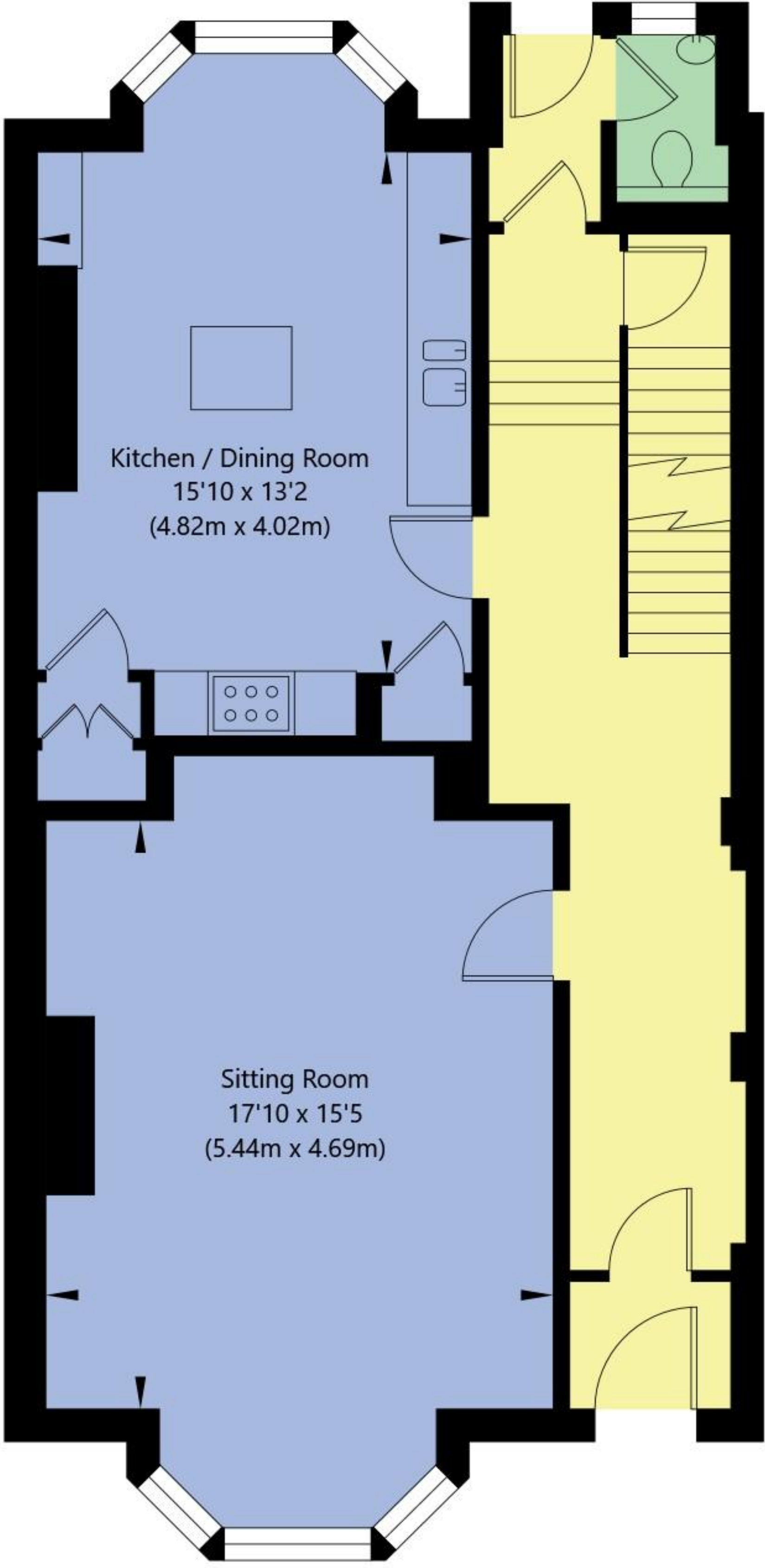
Ground Floor GROSS INTERNAL FLOOR AREA APPROX. 871 SQ FT / 80.91 SQ M
