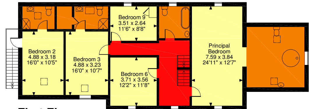
First Floor
